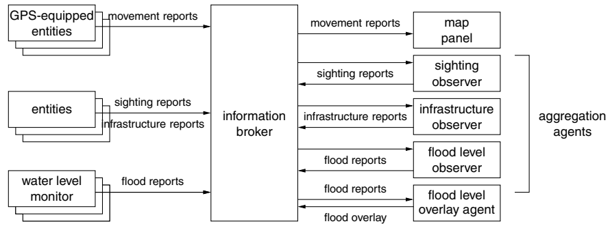
Figure 7: System architecture
