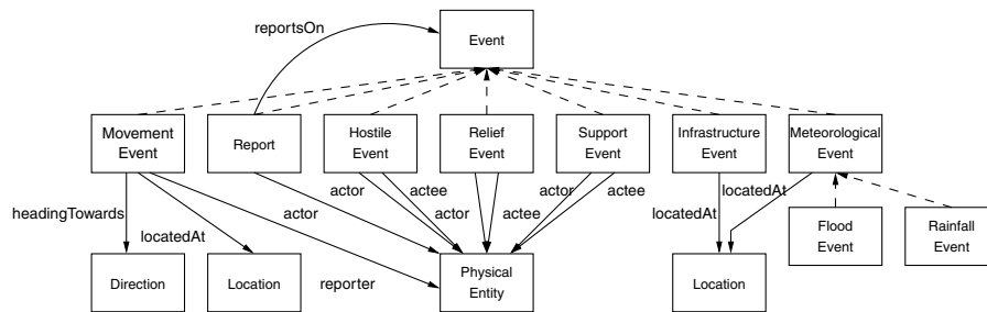
Figure 9: Domain ontology - event
