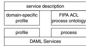
Figure 1: Service Description with ACL Process Ontology
