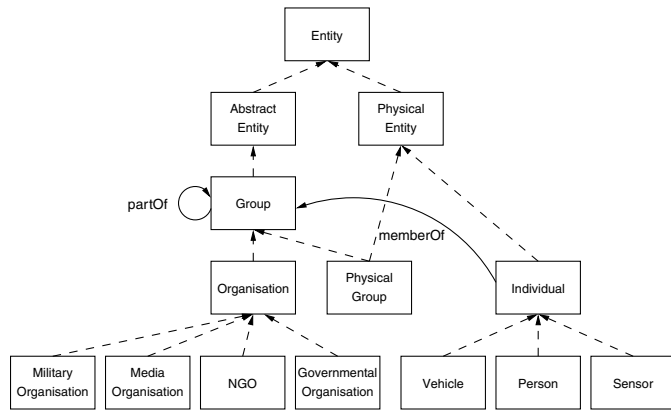
Figure 8: Domain ontology - entity
