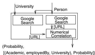
Fig. 10. Example Contextual Instantiation
