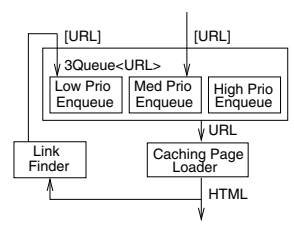
Fig. 5. Example Crawling Instantiation
