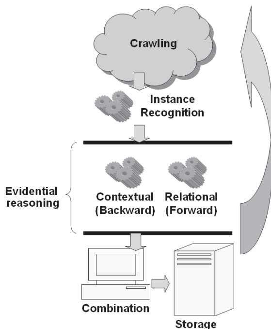
Fig. 1. Harvesting Strategy
