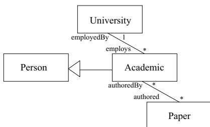
Fig. 2. Example Ontology
