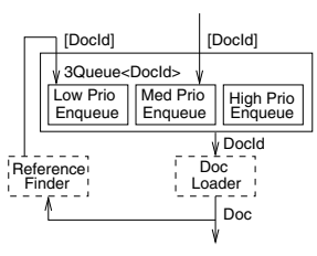
Fig. 4. Crawling Task
