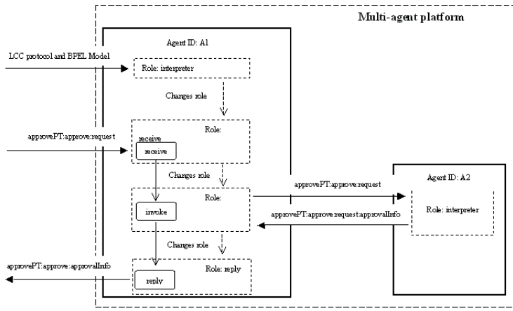
Fig. 7. Agent’s coordination for performing the illustrate example.
