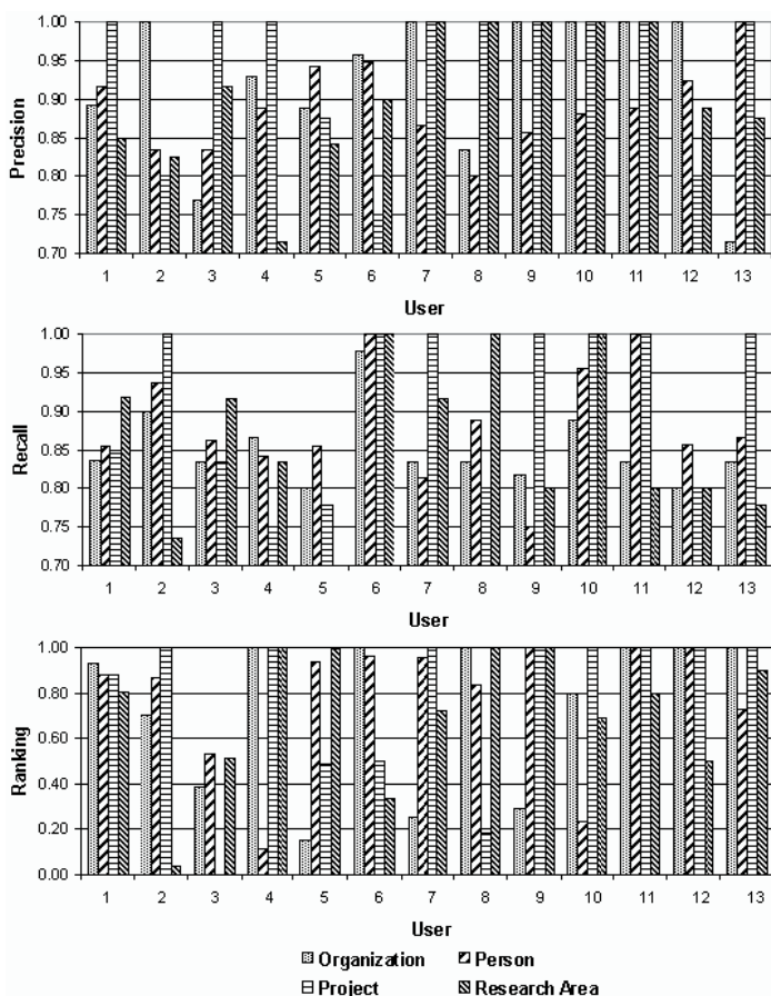
Figure 1: Precision, recall, and ranking accuracy of evaluation
