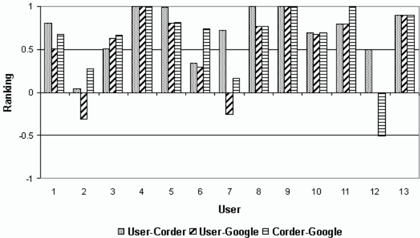
Figure 2. Ranking comparison for users, Google and CORDER
