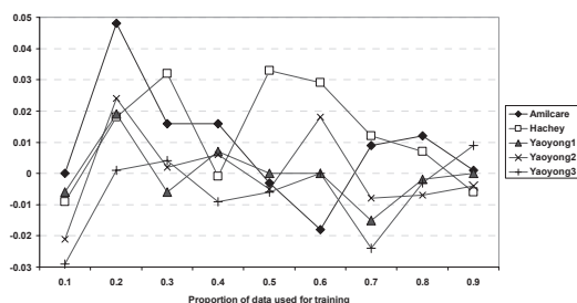
Figure 7: Active Learning Improvement in F-Measure
