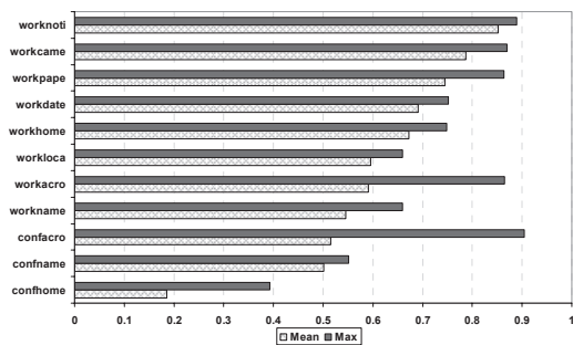
Figure 3: Slot F-Measure for the best systems
