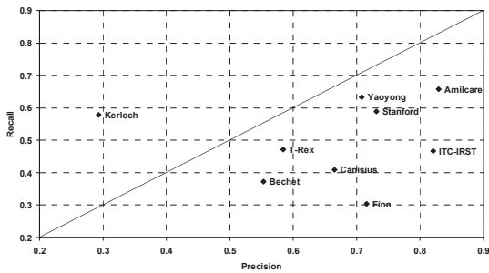
Figure 1: Precision & Recall on Task 1 (Test Corpus)
