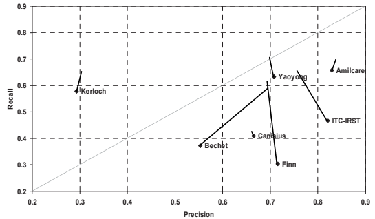
Figure 2: Performance change from 4-fold to test corpus
