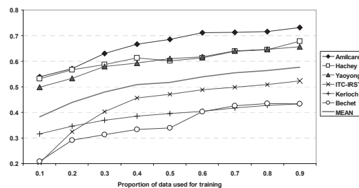
Figure 4: Learning Curve F-Measure
