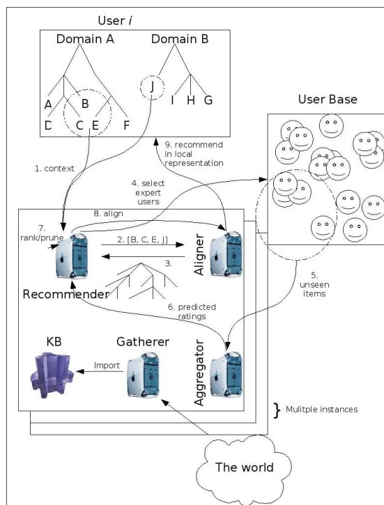
Figure 2: Overview of the recommender system architecture
