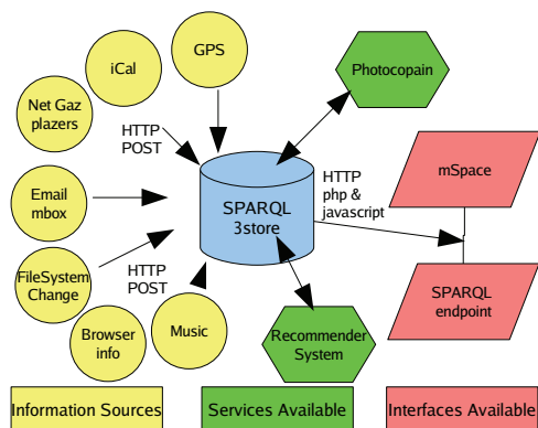
Figure 1: Overview of the Semantic Logger architecture
